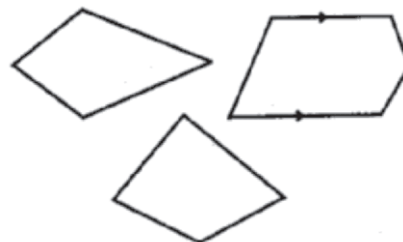
These are not trapeziums
