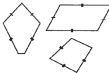
These are not kites
