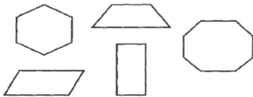
Convex polygons
