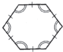
Regular polygons
