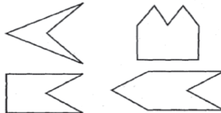
Concave polygons
