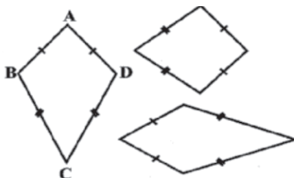
These are kites
