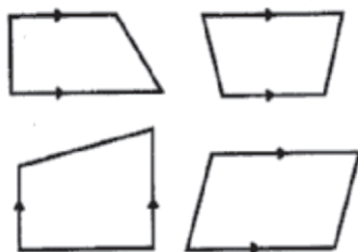
These are trapeziums
