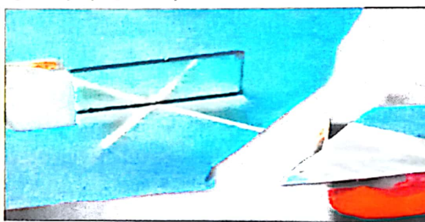
Fig. 11.1 : Arrangement for Showing Reflection
