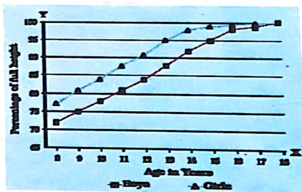
Fig. 10.1 : Graph Showing Percentage of Height with Age
