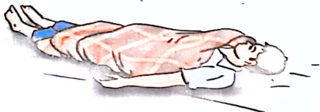
Fig. 7.3 : Blanket Wrapped Around a Person Whose Clothes Caught Fire
