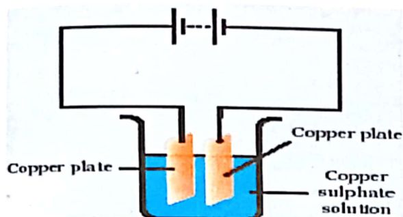
Fig.8.7 : A Simple Circuit Showing Electroplating
