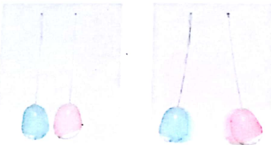
Fig. 13.1 : Like Charges Repel Each Other
