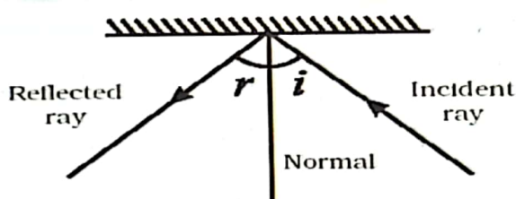
Fig. 11.3 : Angle of Incidence and Angle of Reflection
