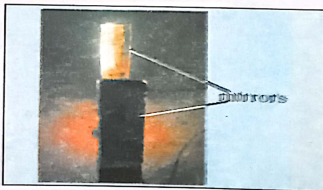
Fig. 11.11 : Images in Plane Mirror Parallel to Each Other
