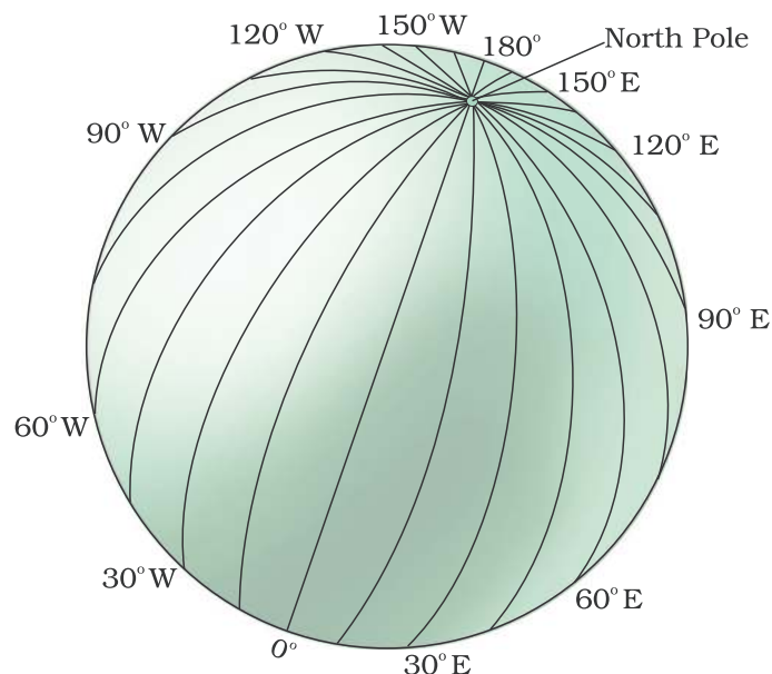
Figure 2.5 : Longitudes
