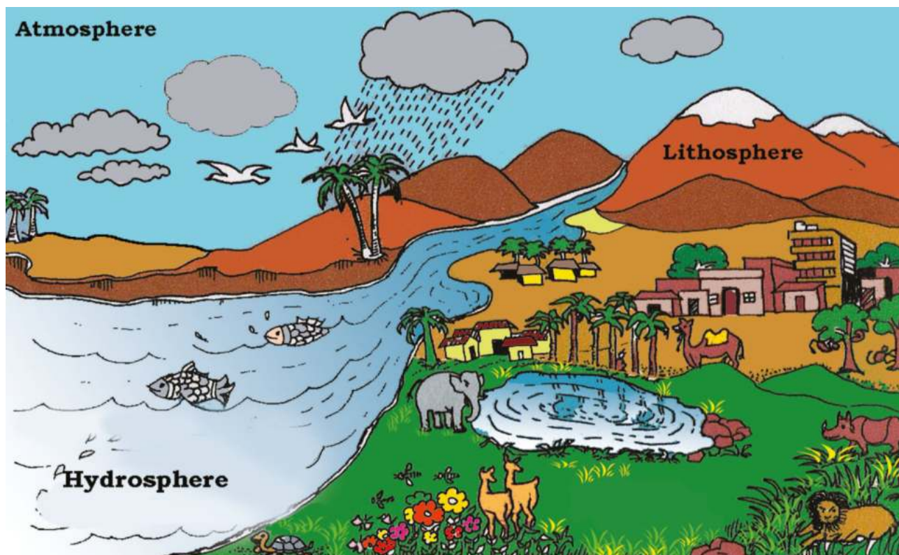
Figure 5.6 : The Biosphere
